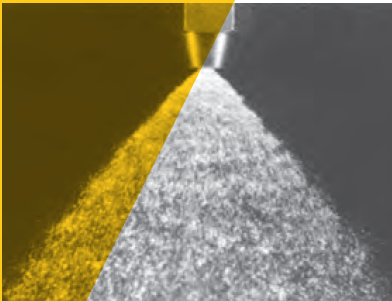
Figure 11: Spray at 100-psi pressure
