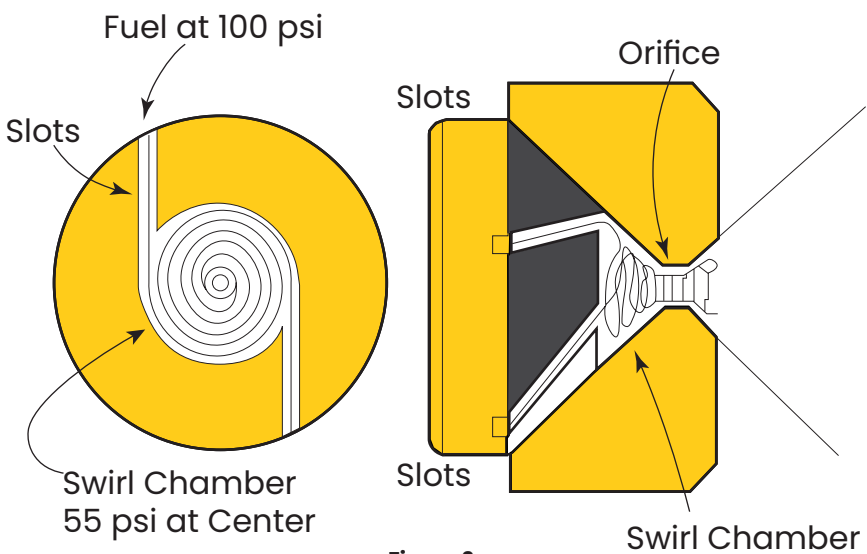
Figure 2: How a nozzle works.
