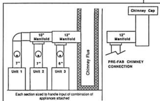
FIGURE 35 Tapered manifold vent system
