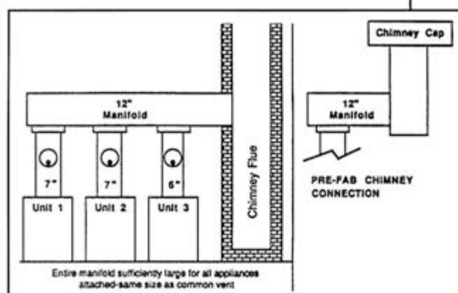
FIGURE 36 Constant sized manifold vent system
