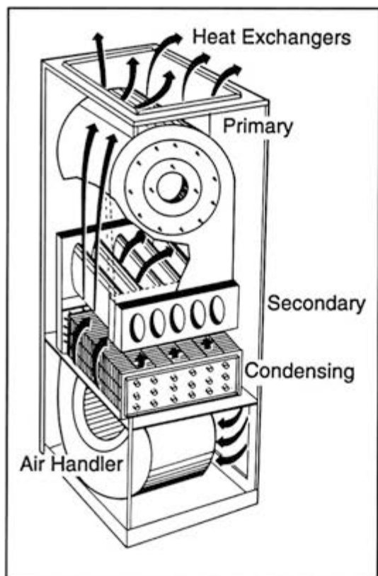
FIGURE 26 Condensing furnace heat exchanger
