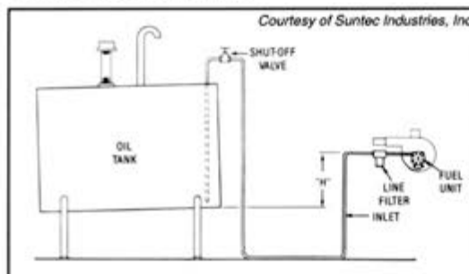
FIGURE 11 Above ground tank
