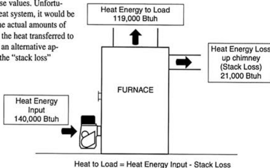
FIGURE 45 Distribution of heat as determined by the stack loss method
