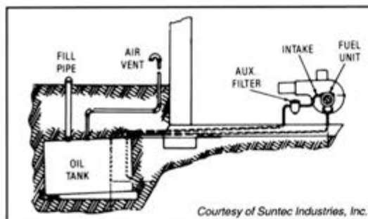
FIGURE 10 Underground tank
