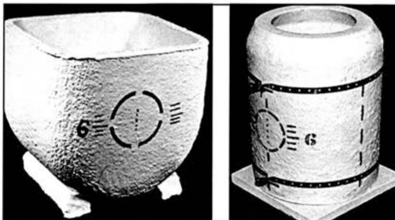
FIGURE 21 Soft fiber refractory combustion chambers
